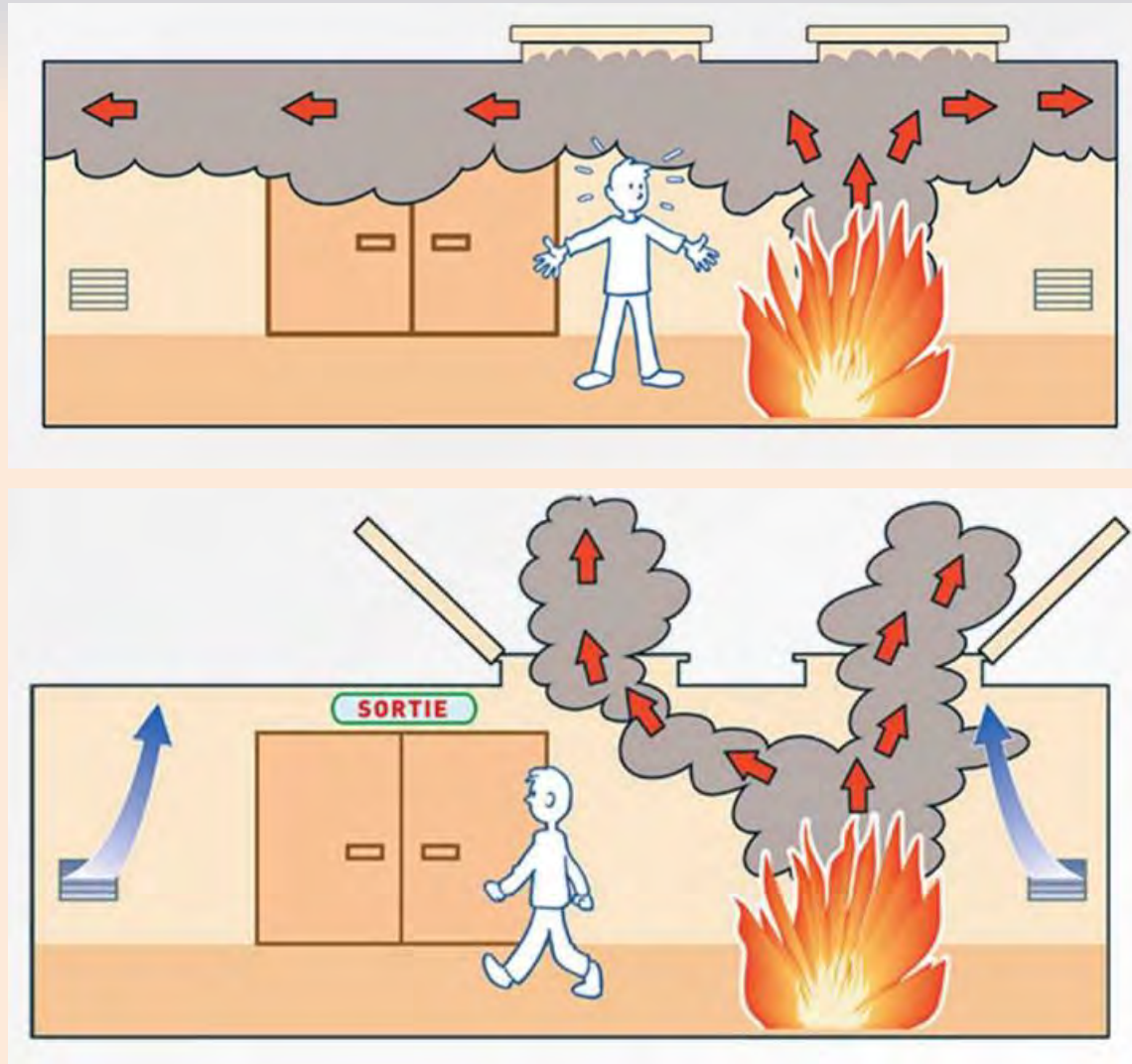
SMOKE SPILL SYSTEM
