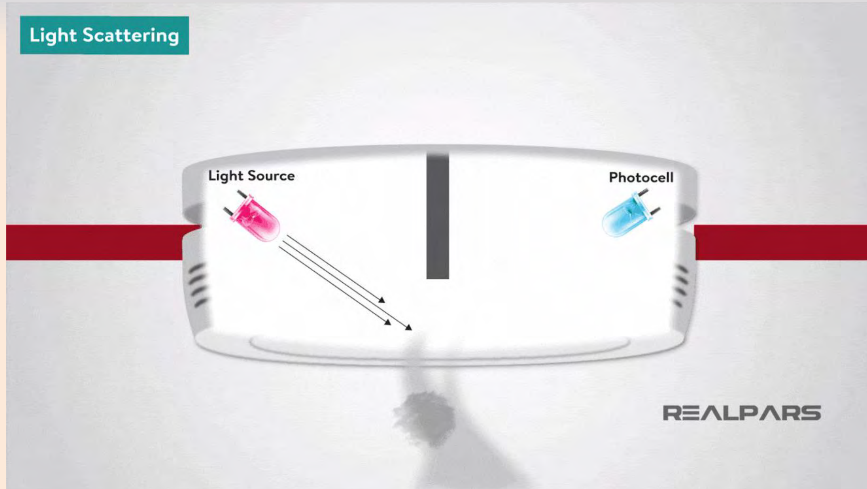
SMOKE DETECTOR
