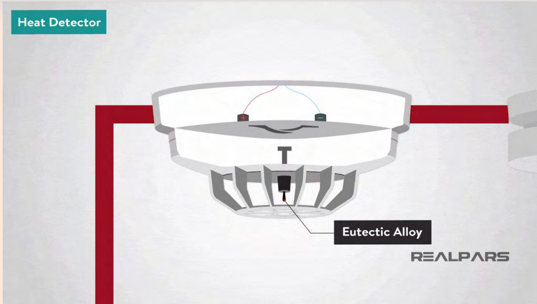
HEAT DETECTOR
