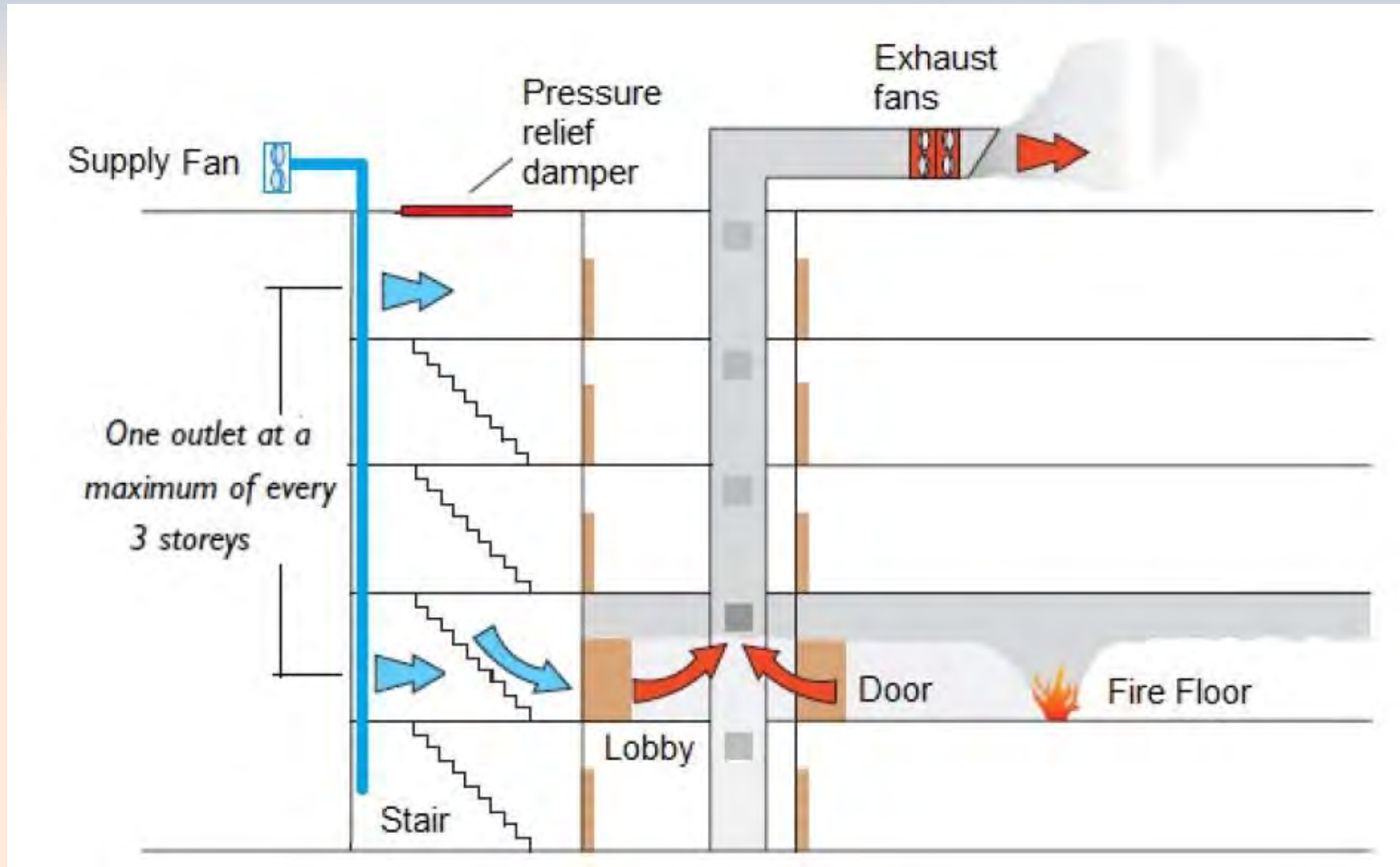
SMOKE SPILL SYSTEM
